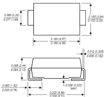
DO-214AA MODIFIED J-BEND
